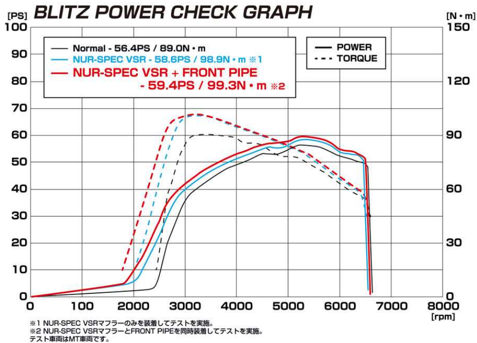
No.21560 Front Pipe
