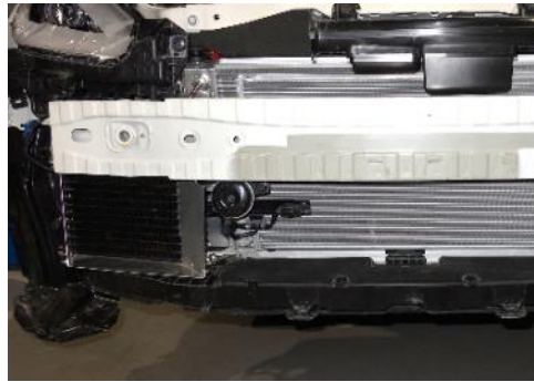
GR86(ZN8) Installation Location
